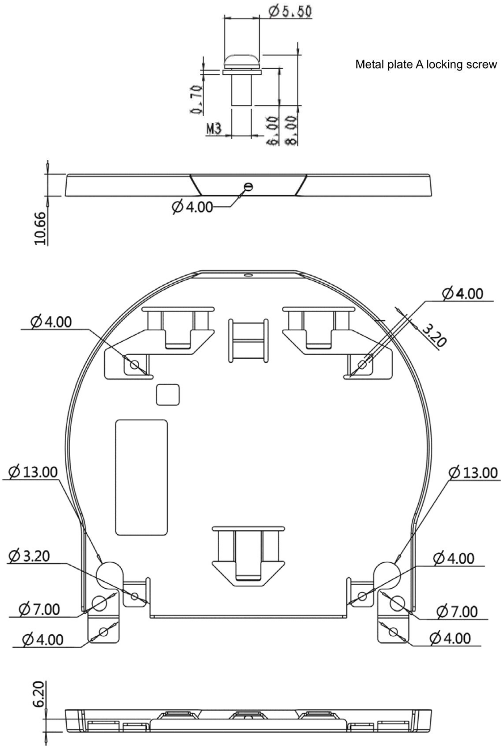
Metal plate A - machine side
